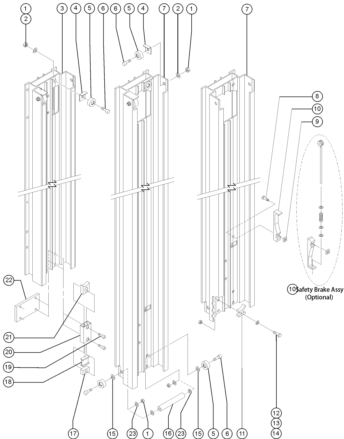
SLA Figure 303.1 Mast Components - View 3
